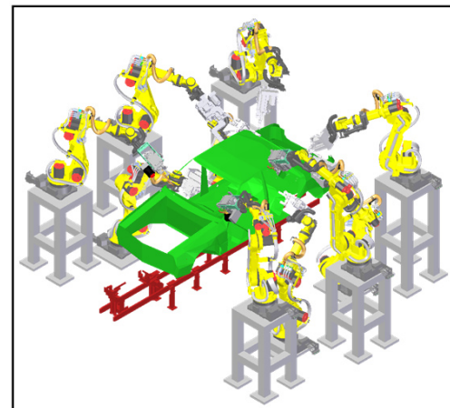
Example of High Density Spot Welding application
